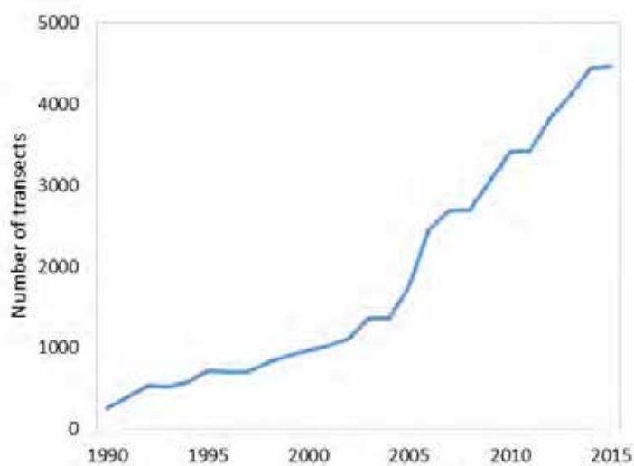
Figure 1: Number of transects used in the European Grassland Butterfly Indicator per year. Since 1990 more than 9200 transects have contributed to the indicator.
