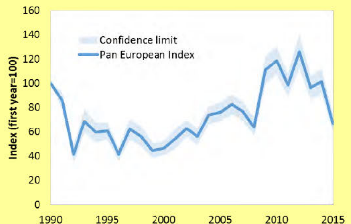
Figure 3: National and Pan-European trends for the Orange Tip ( Anthocharis cardamines ).
