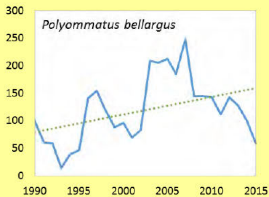
Figure 4: Pan-European population-trends of three butterflies in Europe. The graphs present indices of abundance per year, where 1990 is set to 100. Top: The Wall Brown ( Lasiommata megera ) shows a significant strong decline. Middle: The Dingy Skipper ( Erynnis tages ) is stable. Bottom: In spite of large fluctuations the Adonis Blue ( Polyommatus bellargus ) is increasing.
